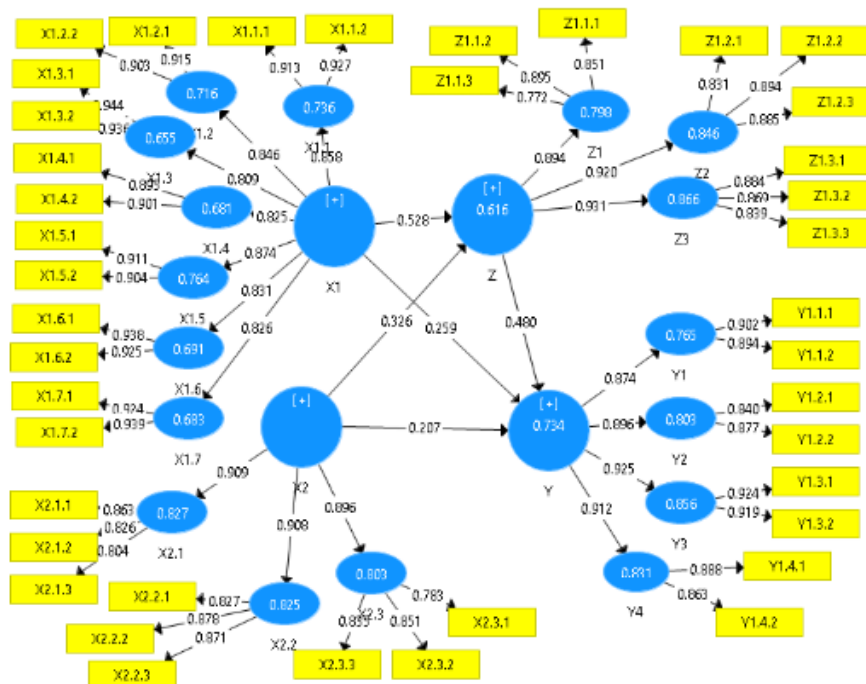
Gambar 1. Outer Model Sumber: Hasil Olah Data (2022)
