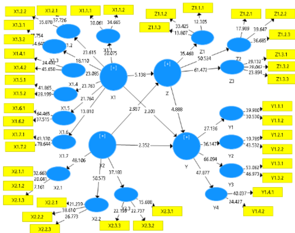
Gambar 2. Inner Model Sumber: Hasil Olah Data (2022)
